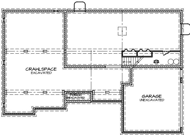
FOUNDATION PLAN A-3
